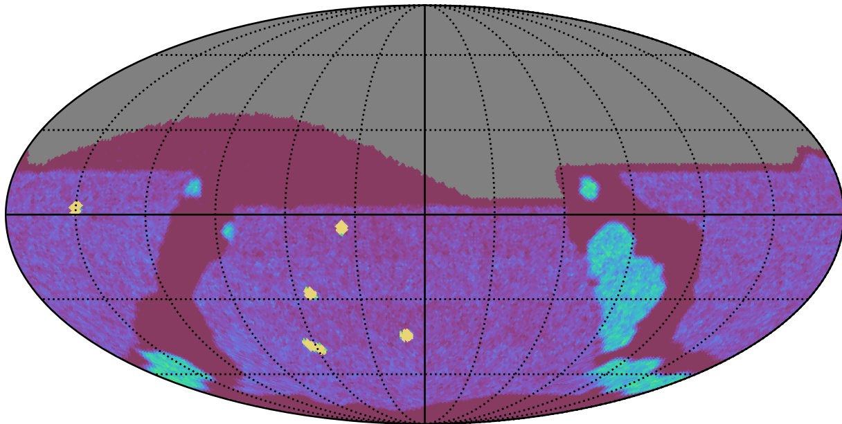
early_ss_template_fpextra3.0_v3.4_10yrs All sky g band: NVisits
