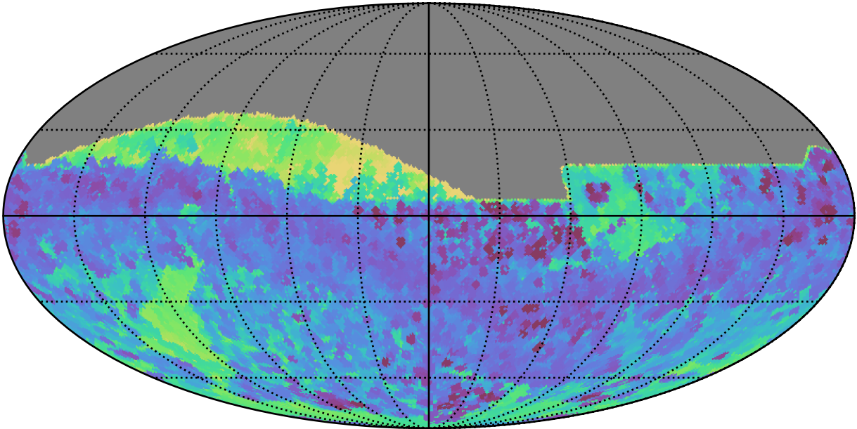
early_ss_template_fpextra3.0_v3.4_10yrs All sky all bands: Min skyBrightness
