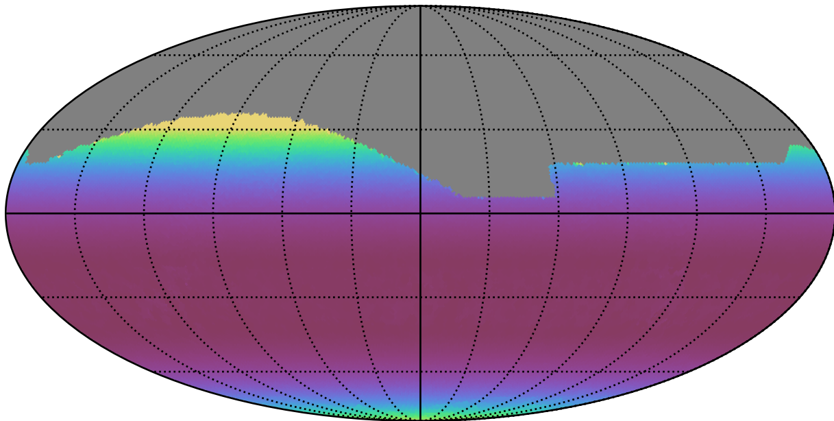
early_ss_template_fpextra3.0_v3.4_10yrs All sky i band: Min airmass
