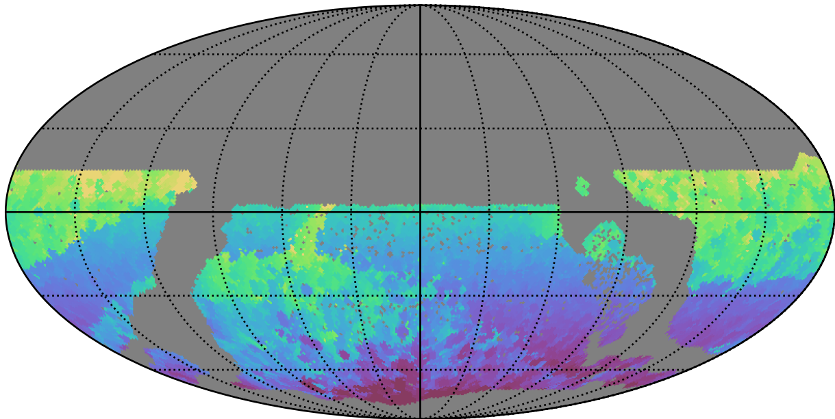
early_ss_template_fpextra3.0_v3.4_10yrs WFD r band: Min HA
