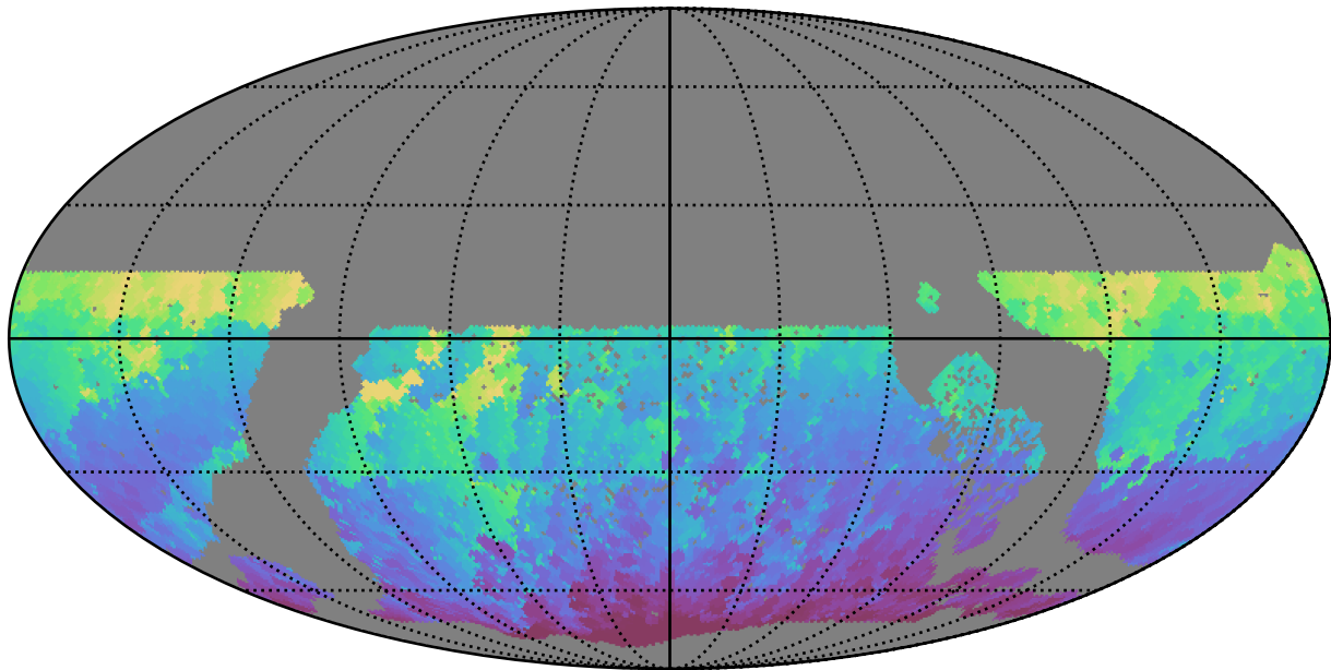
early_ss_template_fpextra3.0_v3.4_10yrs WFD i band: Min HA
