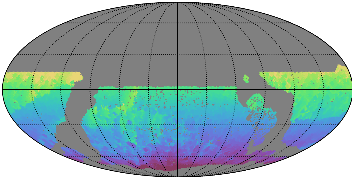
early_ss_template_fpextra3.0_v3.4_10yrs WFD all bands: Min HA
