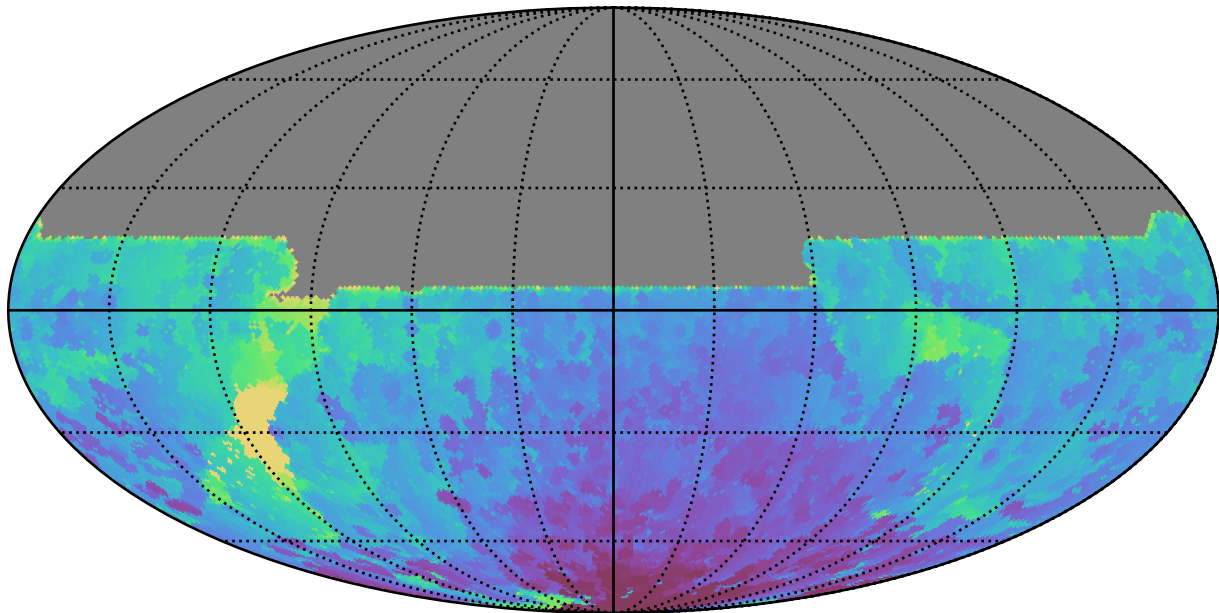
early_ss_template_fpextra3.0_v3.4_10yrs All sky y band: Min HA
