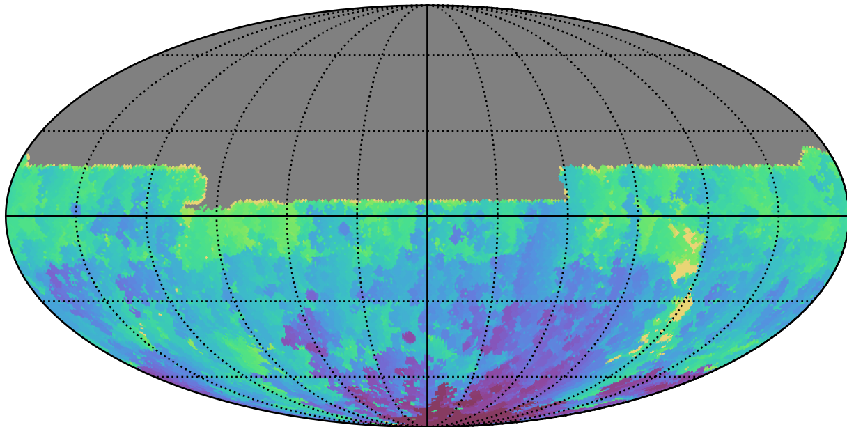
early_ss_template_fpextra3.0_v3.4_10yrs All sky u band: Min HA
