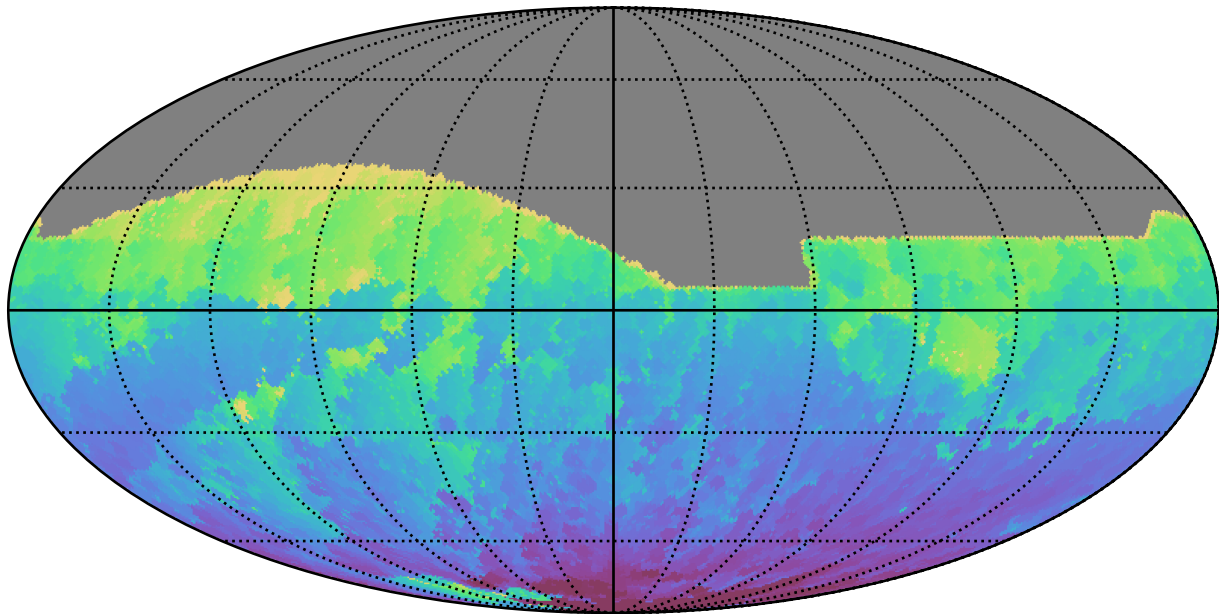
early_ss_template_fpextra3.0_v3.4_10yrs All sky i band: Min HA
