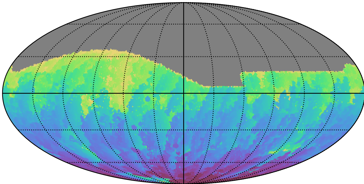
early_ss_template_fpextra3.0_v3.4_10yrs All sky g band: Min HA
