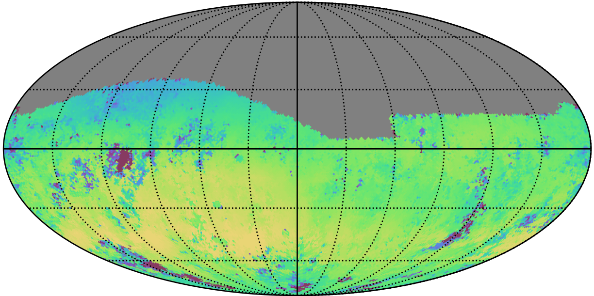
early_ss_template_fpextra3.0_v3.4_10yrs Yr 1 r band: Median skyBrightness
