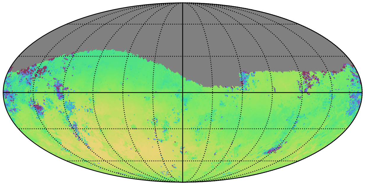
early_ss_template_fpextra3.0_v3.4_10yrs Yr 1 g band: Median skyBrightness
