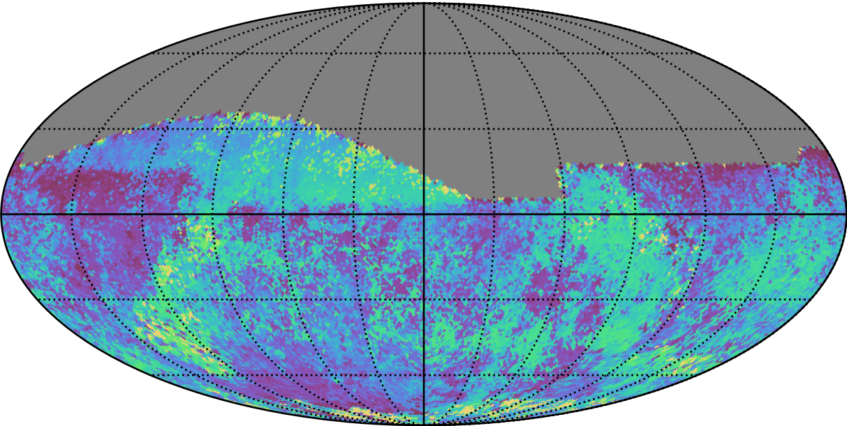
early_ss_template_fpextra3.0_v3.4_10yrs Yr 1 all bands: Median skyBrightness
