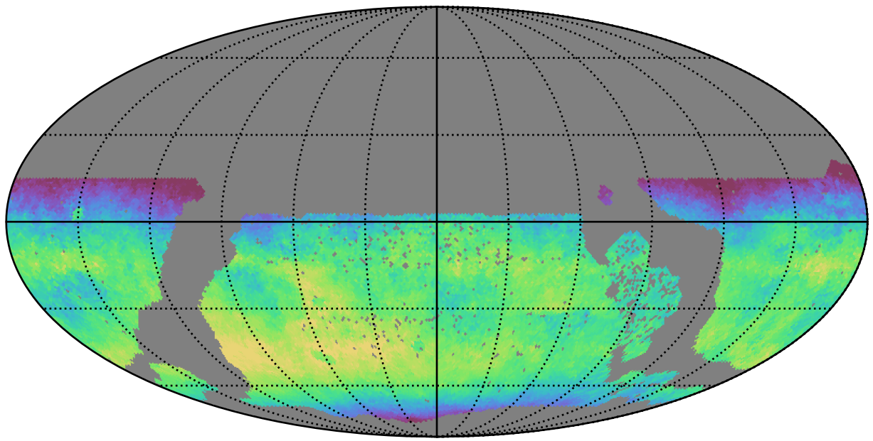
early_ss_template_fpextra3.0_v3.4_10yrs WFD y band: Median skyBrightness
