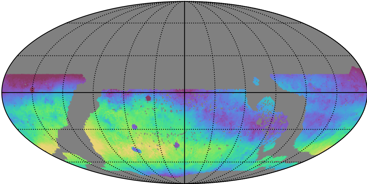
early_ss_template_fpextra3.0_v3.4_10yrs WFD r band: Median skyBrightness
