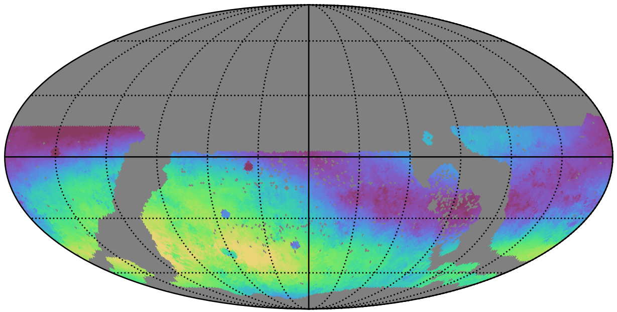
early_ss_template_fpextra3.0_v3.4_10yrs WFD g band: Median skyBrightness
