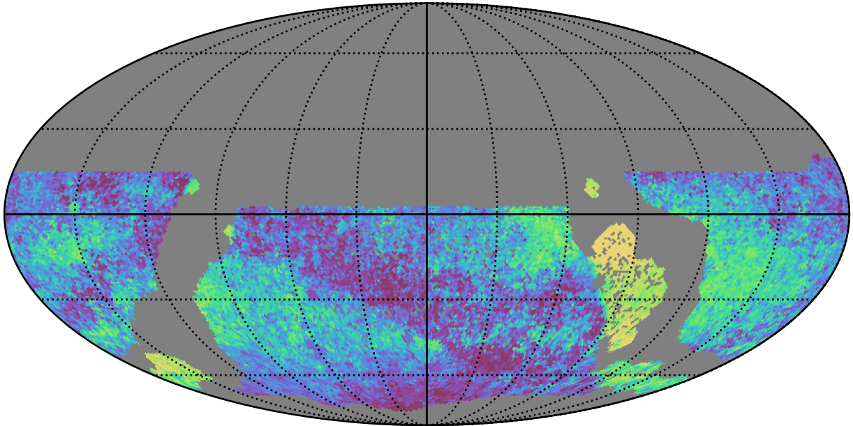
early_ss_template_fpextra3.0_v3.4_10yrs WFD all bands: Median skyBrightness
