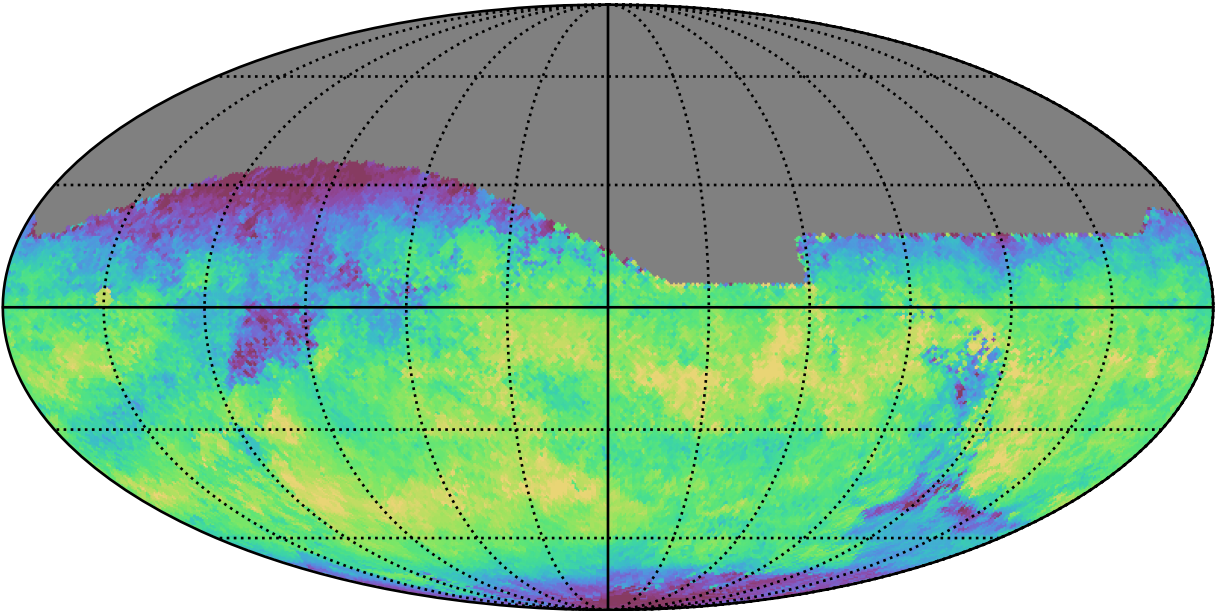
early_ss_template_fpextra3.0_v3.4_10yrs All sky z band: Median skyBrightness
