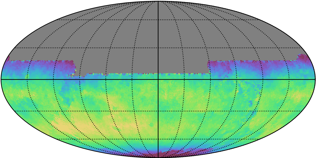
early_ss_template_fpextra3.0_v3.4_10yrs All sky y band: Median skyBrightness
