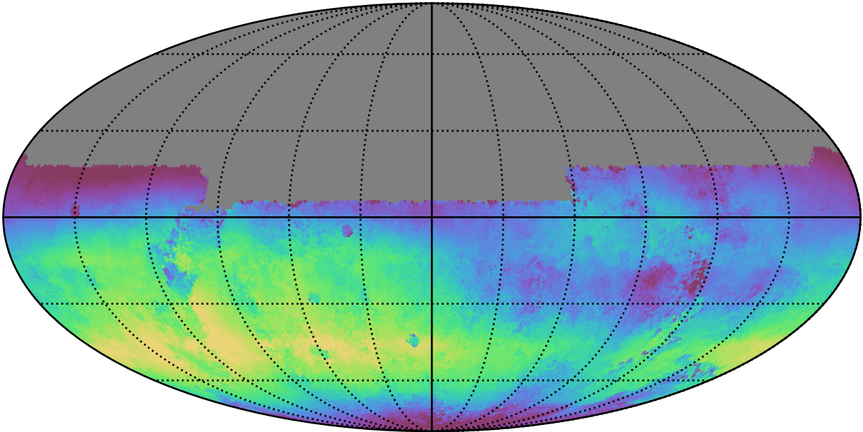
early_ss_template_fpextra3.0_v3.4_10yrs All sky u band: Median skyBrightness
