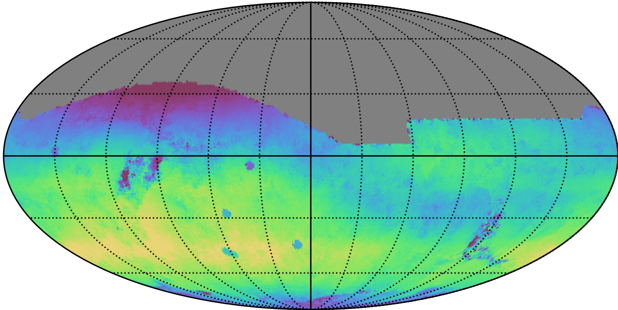
early_ss_template_fpextra3.0_v3.4_10yrs All sky r band: Median skyBrightness
