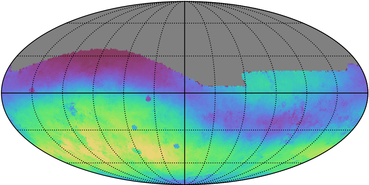
early_ss_template_fpextra3.0_v3.4_10yrs All sky g band: Median skyBrightness
