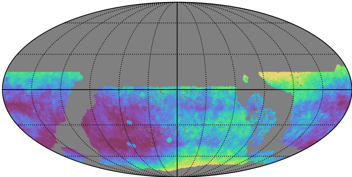
early_ss_template_fpextra3.0_v3.4_10yrs WFD i band: Median seeingEff
