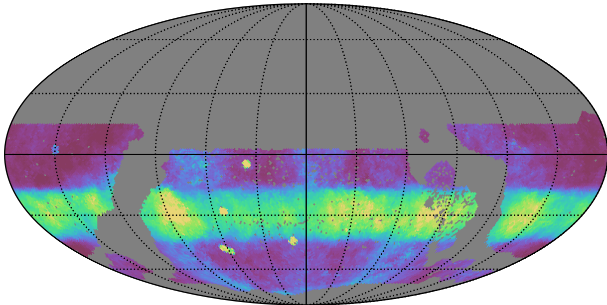
early_ss_template_fpextra3.0_v3.4_10yrs WFD r band: Median normairmass
