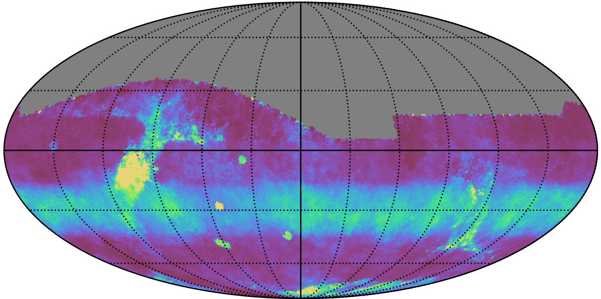
early_ss_template_fpextra3.0_v3.4_10yrs All sky z band: Median normairmass
