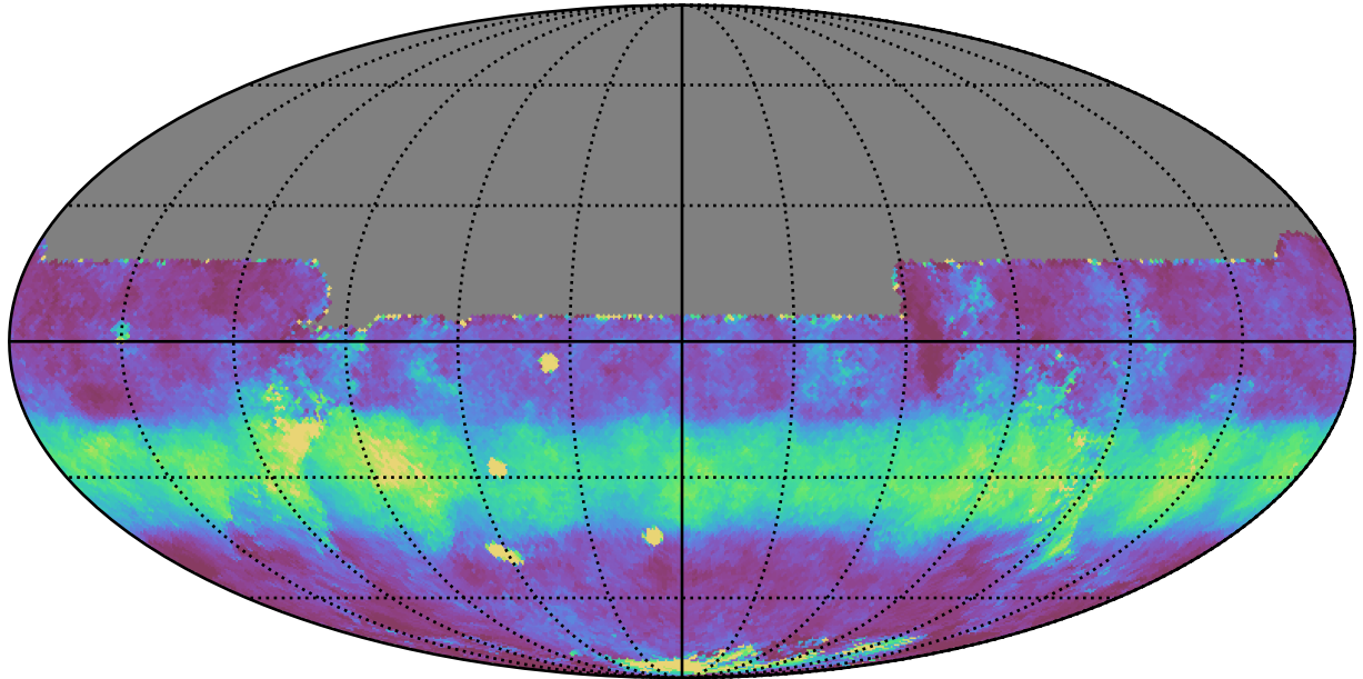
early_ss_template_fpextra3.0_v3.4_10yrs All sky y band: Median normairmass
