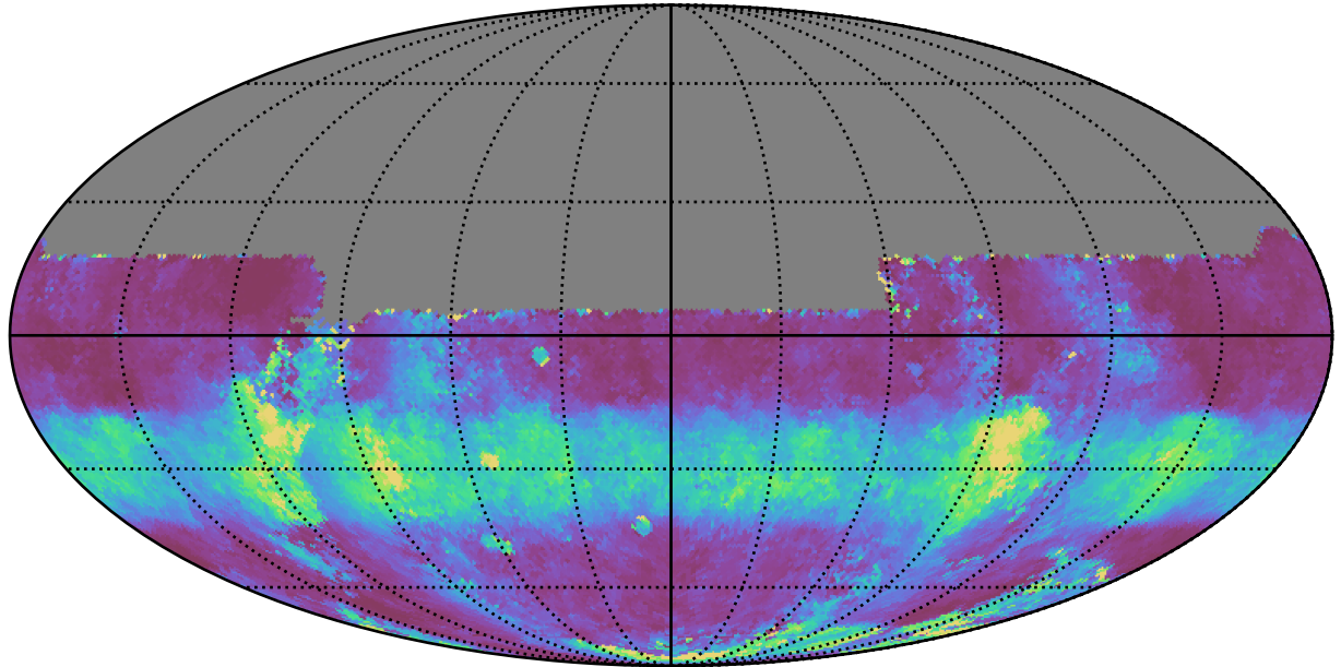
early_ss_template_fpextra3.0_v3.4_10yrs All sky u band: Median normairmass
