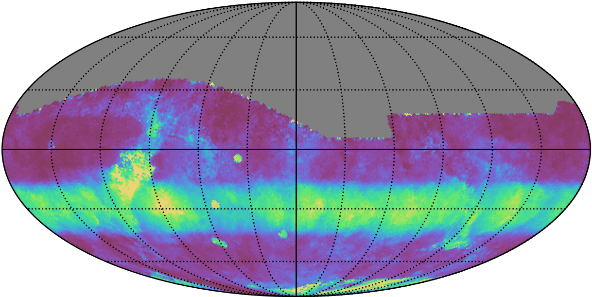
early_ss_template_fpextra3.0_v3.4_10yrs All sky i band: Median normairmass
