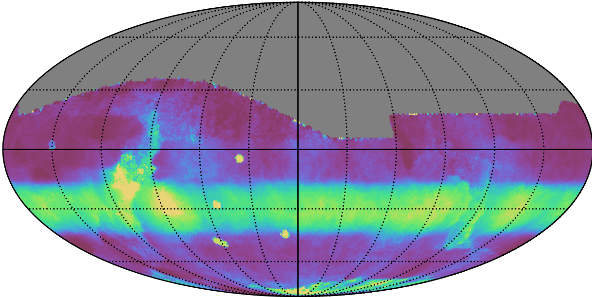
early_ss_template_fpextra3.0_v3.4_10yrs All sky all bands: Median normairmass
