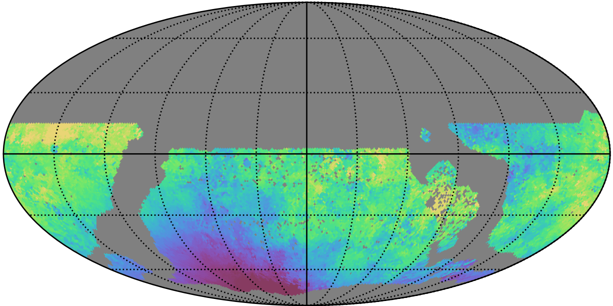
early_ss_template_fpextra3.0_v3.4_10yrs WFD u band: Median moonDistance
