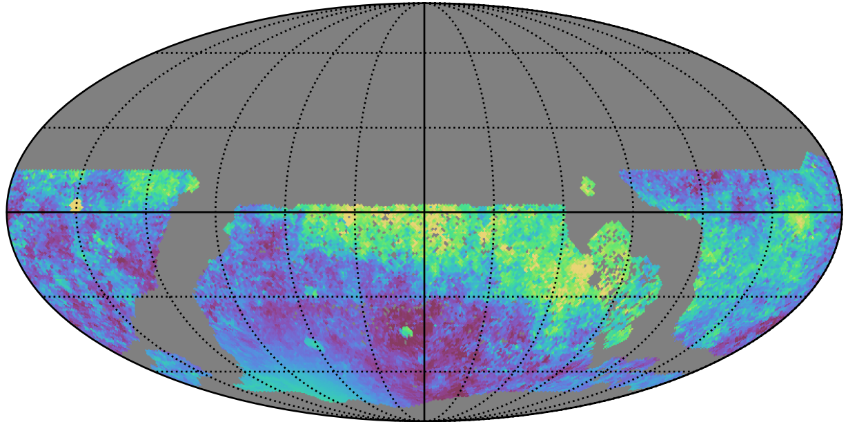
early_ss_template_fpextra3.0_v3.4_10yrs WFD all bands: Median moonDistance
