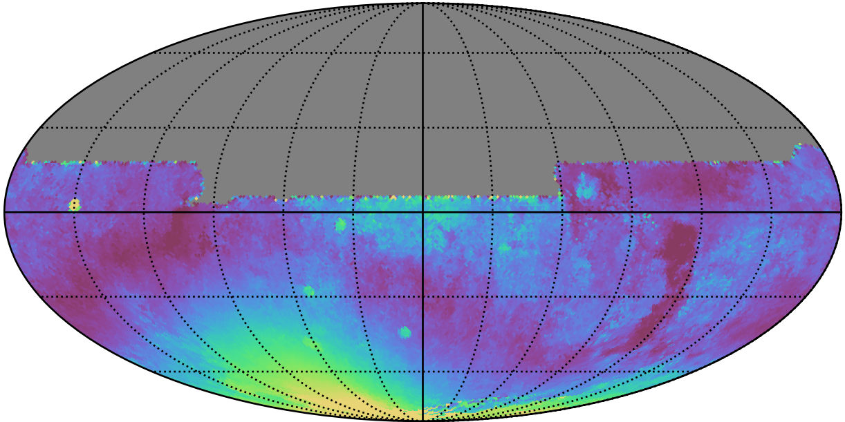
early_ss_template_fpextra3.0_v3.4_10yrs All sky y band: Median moonDistance
