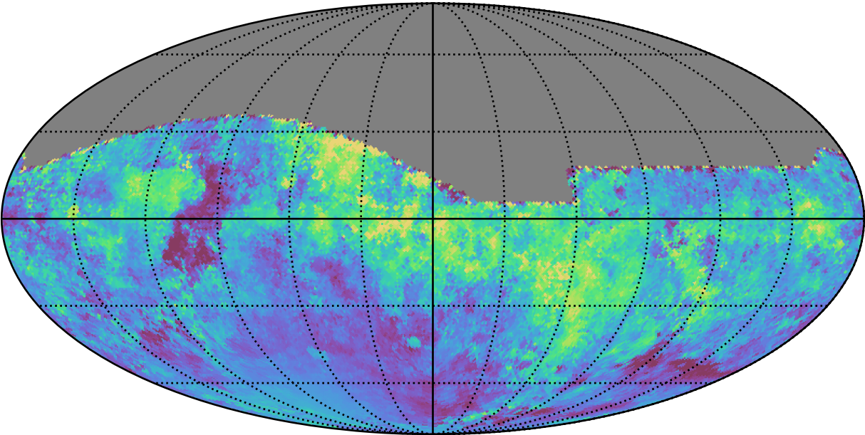
early_ss_template_fpextra3.0_v3.4_10yrs All sky i band: Median moonDistance
