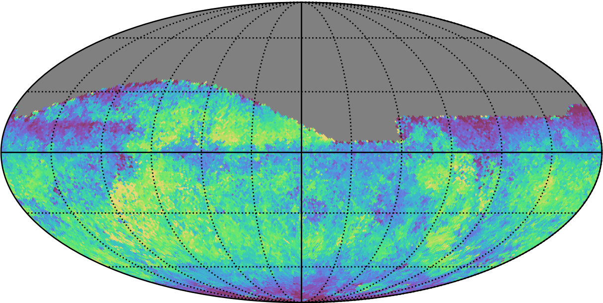
early_ss_template_fpextra3.0_v3.4_10yrs Yr 1 all bands: Median fiveSigmaDepth
