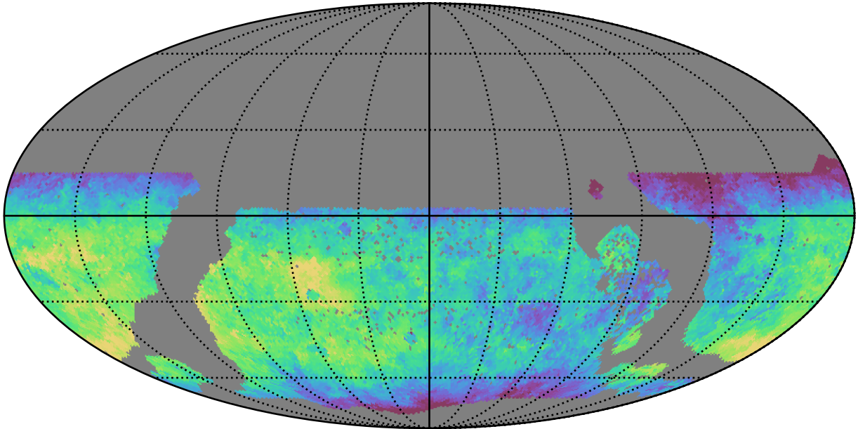
early_ss_template_fpextra3.0_v3.4_10yrs WFD u band: Median fiveSigmaDepth
