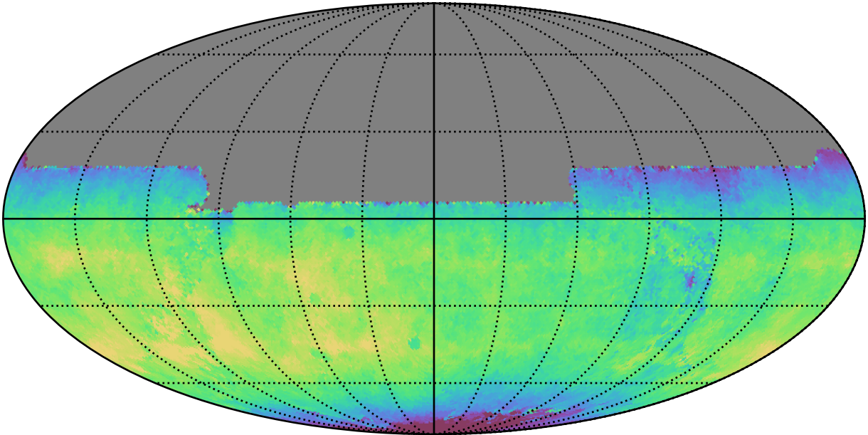
early_ss_template_fpextra3.0_v3.4_10yrs All sky y band: Median fiveSigmaDepth
