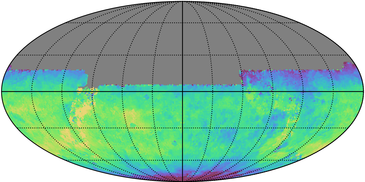
early_ss_template_fpextra3.0_v3.4_10yrs All sky u band: Median fiveSigmaDepth
