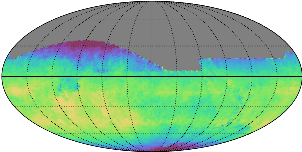
early_ss_template_fpextra3.0_v3.4_10yrs All sky i band: Median fiveSigmaDepth
