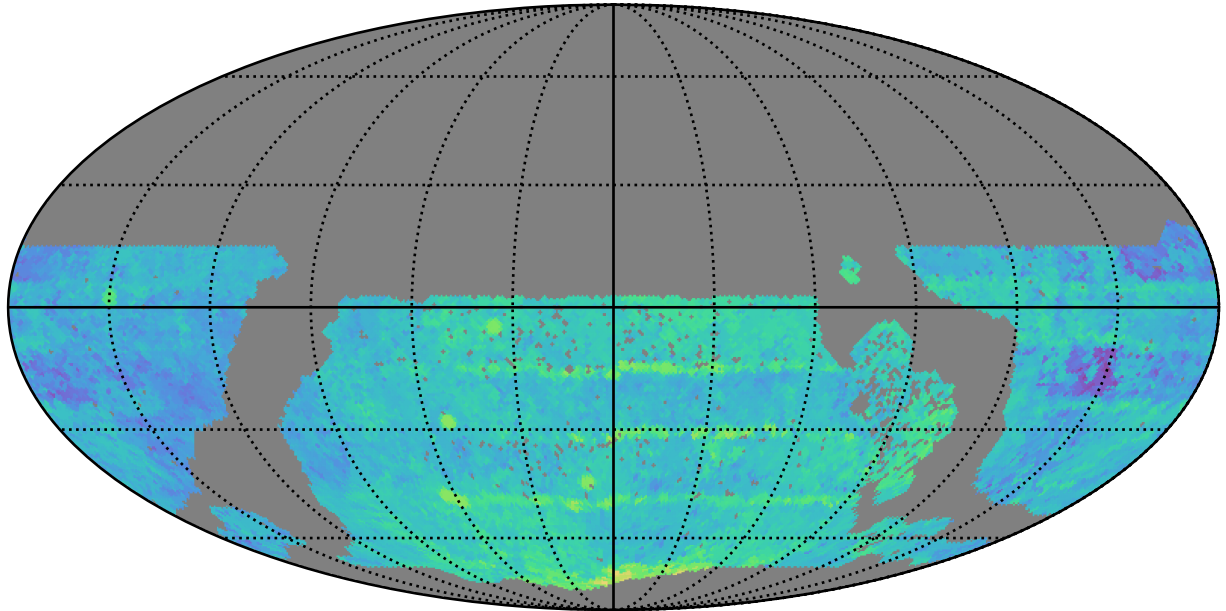
early_ss_template_fpextra3.0_v3.4_10yrs WFD z band: Median Season Length
