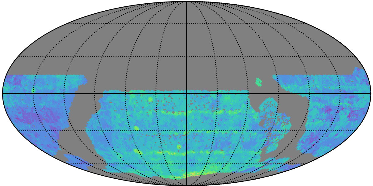
early_ss_template_fpextra3.0_v3.4_10yrs WFD y band: Median Season Length
