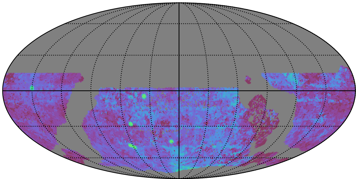
early_ss_template_fpextra3.0_v3.4_10yrs WFD u band: Median Season Length
