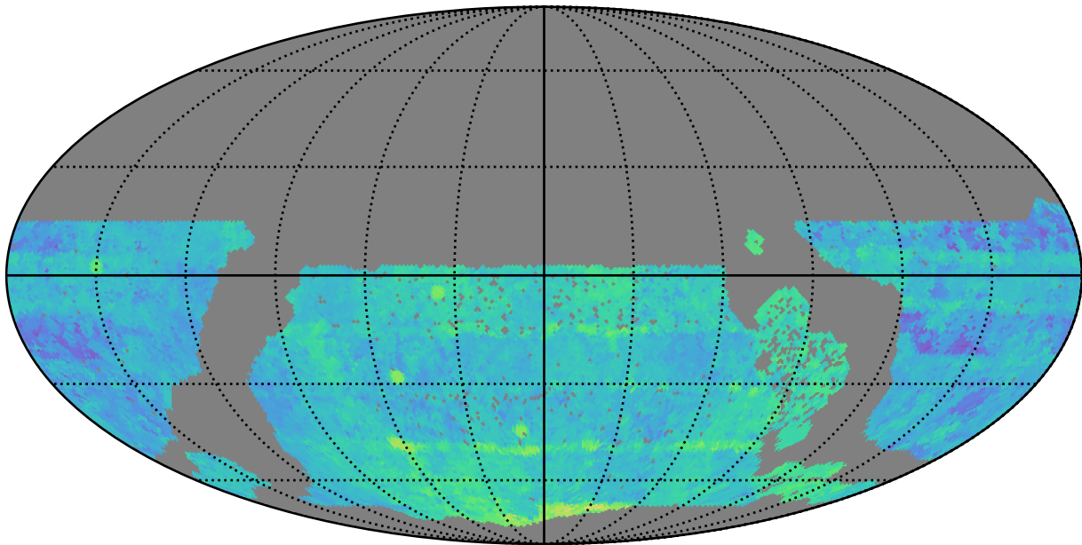
early_ss_template_fpextra3.0_v3.4_10yrs WFD i band: Median Season Length
