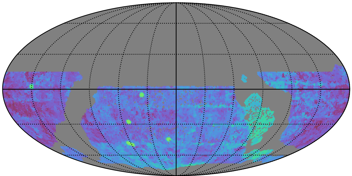
early_ss_template_fpextra3.0_v3.4_10yrs WFD g band: Median Season Length
