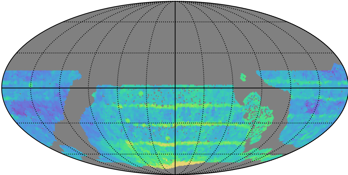
early_ss_template_fpextra3.0_v3.4_10yrs WFD all bands: Median Season Length
