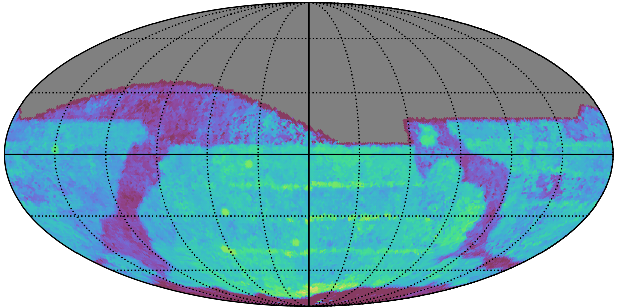
early_ss_template_fpextra3.0_v3.4_10yrs All sky z band: Median Season Length
