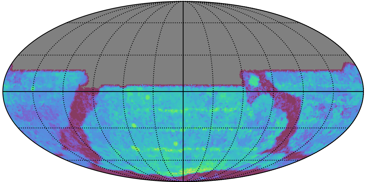
early_ss_template_fpextra3.0_v3.4_10yrs All sky y band: Median Season Length
