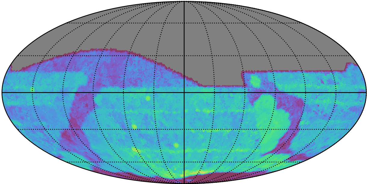
early_ss_template_fpextra3.0_v3.4_10yrs All sky r band: Median Season Length
