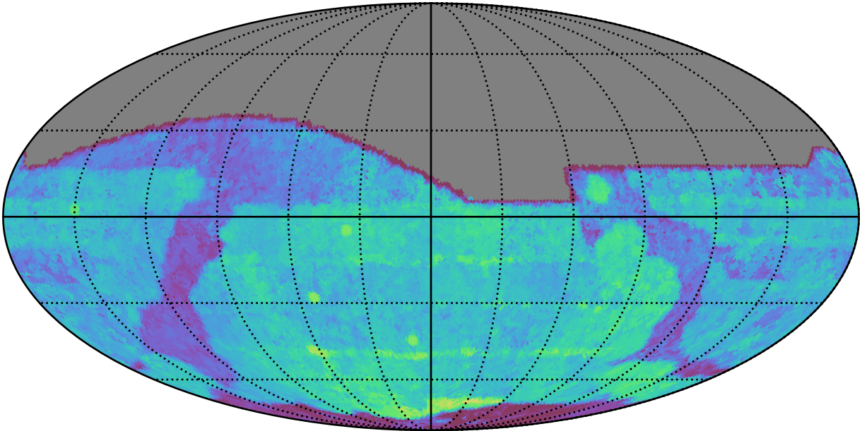
early_ss_template_fpextra3.0_v3.4_10yrs All sky i band: Median Season Length
