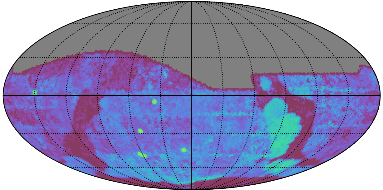
early_ss_template_fpextra3.0_v3.4_10yrs All sky g band: Median Season Length
