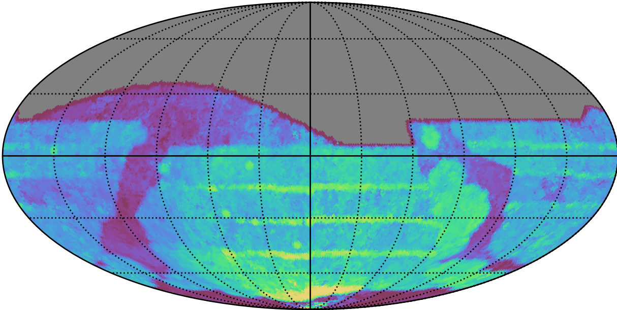
early_ss_template_fpextra3.0_v3.4_10yrs All sky all bands: Median Season Length
